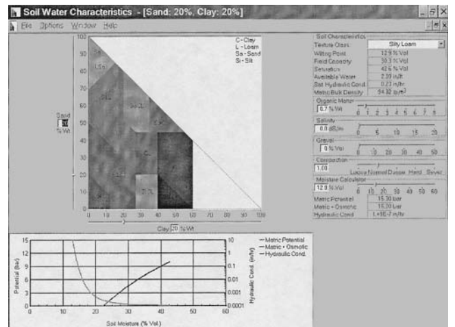
Fig. 11. Graphical input screen for the soil water characteristic model of Table 1 equations.
