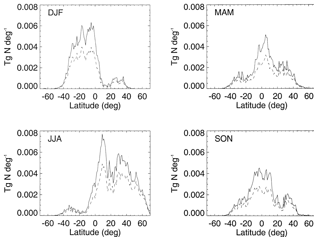
Fig. 3. Quarterly latitudinal distribution of lightning produced \text{NO}_x (presented in \text{Tg N per } 1.0^\circ ). Dashed lines indicate contribution from CG flashes; the portion from the dashed lines to the solid lines corresponds to the contribution from IC flashes.
