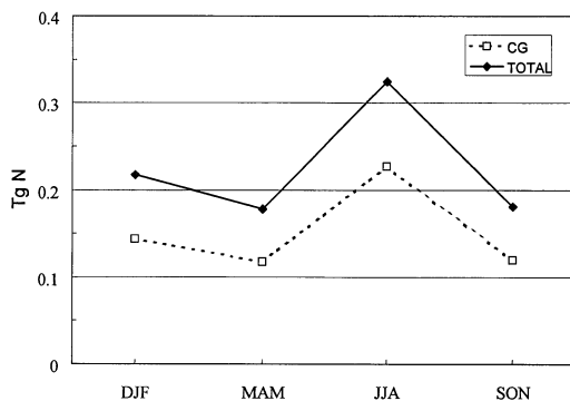
Fig. 1. \text{NO}_x production by IC and CG lightning in \text{Tg N} is shown quarterly (i.e., DJF, MAM, JJA, and SON) in 1996. The dashed line indicates contribution from CG flashes; the portion from the dashed line to the solid line corresponds to the contribution from IC flashes.
