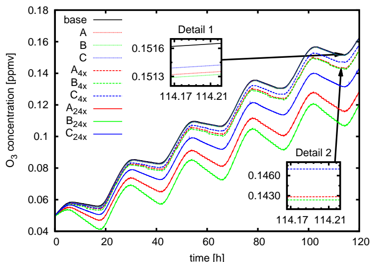
Fig. 7. The temporal evolution of the gas-phase O 3 concentration is shown for a base scenario with no heterogeneous chemistry, for the model scenarios A, B, C, and the corresponding low and high emission scenarios A 4x , B 4x , C 4x and A 24x , B 24x , C 24x , respectively. Detail 1 shows an enlarged view of the results of the base scenario and model scenarios A, B, and C. Detail 2 shows an enlarged view of the results for the low emissions scenarios A 4x , B 4x , C 4x . Input parameters for the A, B, and C-scenarios are given in Table 1.
