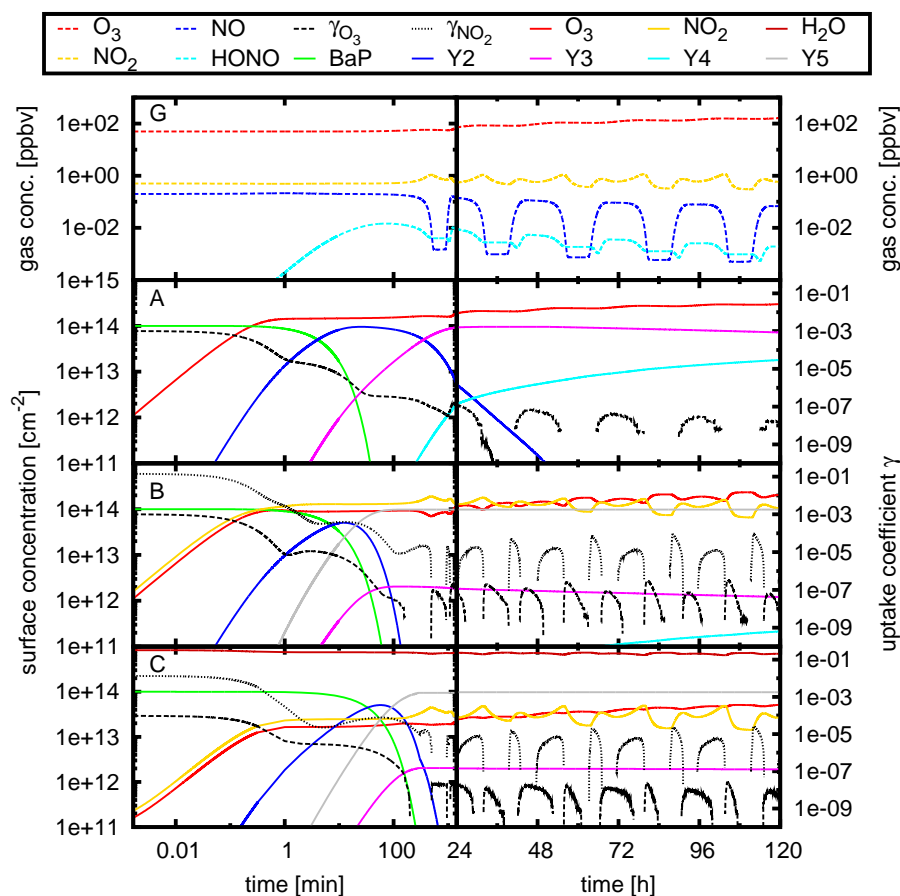
Fig. 2. The temporal evolution of gas-phase component concentrations ( G ), surface component concentrations, and uptake coefficients for the adsorption and surface reaction of O 3 ( A ), the co-adsorption of O 3 and NO 2 ( B ), and the co-adsorption of O 3 , NO 2 , and H 2 O ( C ) following the surface reactions defined in Table 1 is plotted on a logarithmic timescale for day one (left panels) and on a linear timescale for the four following days (right panels).
