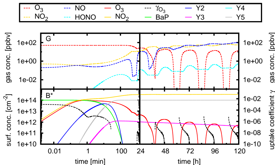
Fig. 4. The temporal evolution of gas-phase component concentrations (G), surface component concentrations, and uptake coefficients for scenario B* are shown and plotted on a logarithmic timescale for day one (left panels) and on a linear timescale for the four following days (right panels). Scenario B* corresponds to scenario B with a 10-fold increase of the NO emission rates.
