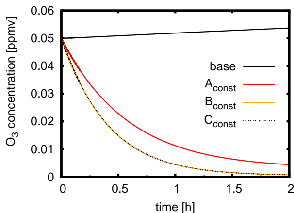
Fig. 8. The temporal evolution of the gas-phase O 3 concentration is shown for a base scenario with no heterogeneous chemistry and for the constant uptake scenarios A const , B const , C const . Scenarios A const , B const , C const use constant uptake coefficients of \gamma_{\text{O}_3}=1\times 10^{-3} (Stephens et al., 1986; Pöschl et al., 2001), \gamma_{\text{NO}_2}=0.14 (Gerecke et al., 1998; Ammann and Pöschl, 2007), and \gamma_{\text{H}_2\text{O}}=0.4\times 10^{-3} (Rogaski et al., 1997; Pöschl et al., 2001) but are otherwise equivalent to scenarios A, B, and C as defined in Table 1.
