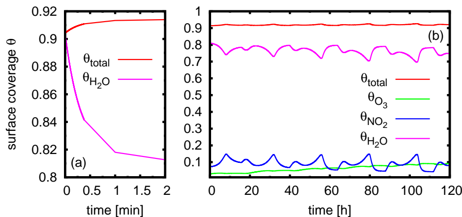
Fig. 3. The temporal evolution of the soot surface coverage \theta in scenario C is shown for the first 2 min (a), and for the entire simulation period of five days (b). The total surface coverage is indicated by \theta_{\text{total}} , and the fractional surface coverages of O 3 , NO 2 , and H 2 O by \theta_{\text{O}_3} , \theta_{\text{NO}_2} , and \theta_{\text{H}_2\text{O}} , respectively. Input parameters and surface reactions for scenario C are given in Table 1.
