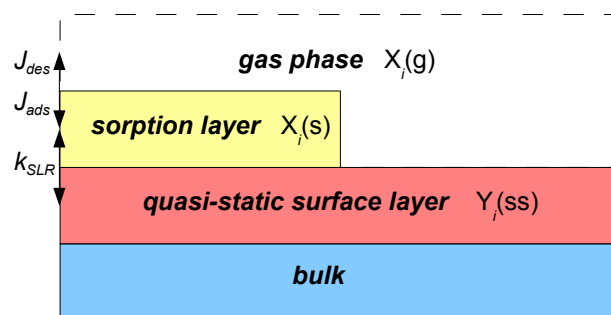
Fig. 1. The applied surface layer model is shown as a schematic. The gas-particle interface is divided into a gas-phase (g) with gas-phase species X_i(g) , a sorption layer (s) with adsorbed gas-phase species X_i(s) , a quasi-static surface layer (ss) with non-volatile particle components Y_i(ss) , and a particle bulk. The adsorption and desorption fluxes are indicated as J_{ads} and J_{des} , respectively, and the rate coefficient for surface layer reactions is denoted by k_{SLR} . Adapted from Pöschl et al. (2007).
