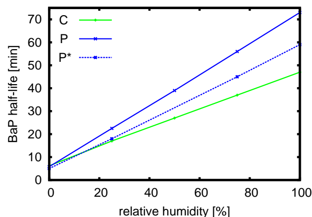
Fig. 6. The BaP half-life is plotted as a function of relative humidity for scenarios C, P, and P*. Scenario C represents the co-adsorption of O 3 , NO 2 , and H 2 O following the surface reactions given in Table 1 with an initial gas-phase O 3 concentration of 50 ppbv, an initial BaP surface concentration of 1 \times 10^{14} \text{ cm}^{-2} , and a temperature of 298.15 K. Scenario P represents the co-adsorption of O 3 and H 2 O following surface Reactions (R1) to (R3) from Table 1 with a constant gas-phase O 3 concentration of 30 ppbv, an initial BaP surface concentration of 1.8 \times 10^{13} \text{ cm}^{-2} , and a temperature of 296 K corresponding to the boundary conditions of an aerosol flow tube experiment conducted by Pöschl et al. (2001). Scenario P* represents the experimentally derived BaP half-lives from the aerosol flow tube experiment (Pöschl et al., 2001) with the same boundary conditions as used in scenario P.
