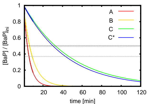
Fig. 5. The temporal evolution of the ratio of actual BaP surface concentration to initial BaP concentration is shown for scenarios A, B, C, and C*. Scenario A represents the adsorption of O 3 , scenario B the co-adsorption of O 3 and NO 2 , scenario C the co-adsorption of O 3 , NO 2 , and H 2 O, and scenario C* the co-adsorption of O 3 and H 2 O. Scenarios A, B, and C follow the surface reactions given in Table 1; scenario C* follows the surface reactions (R1) to (R3) given in Table 1. The intersection with the horizontal dotted lines indicate BaP half-life (dotted black line) and BaP lifetime (dotted grey line).
